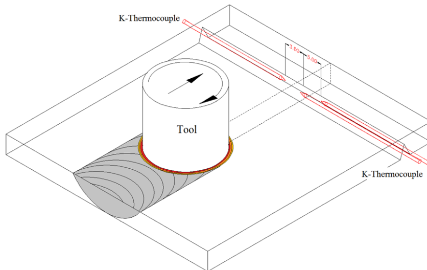
Fig. 3. The thermocouple set up
