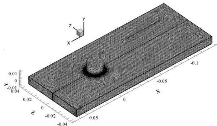
Fig. 2. The meshed model of the process
