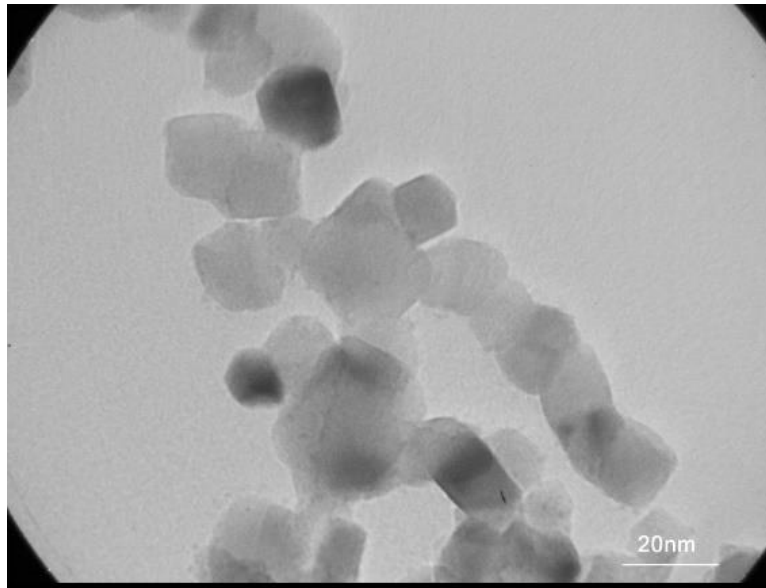
Fig. 3: TEM image of TiO 2 nanoparticles.
