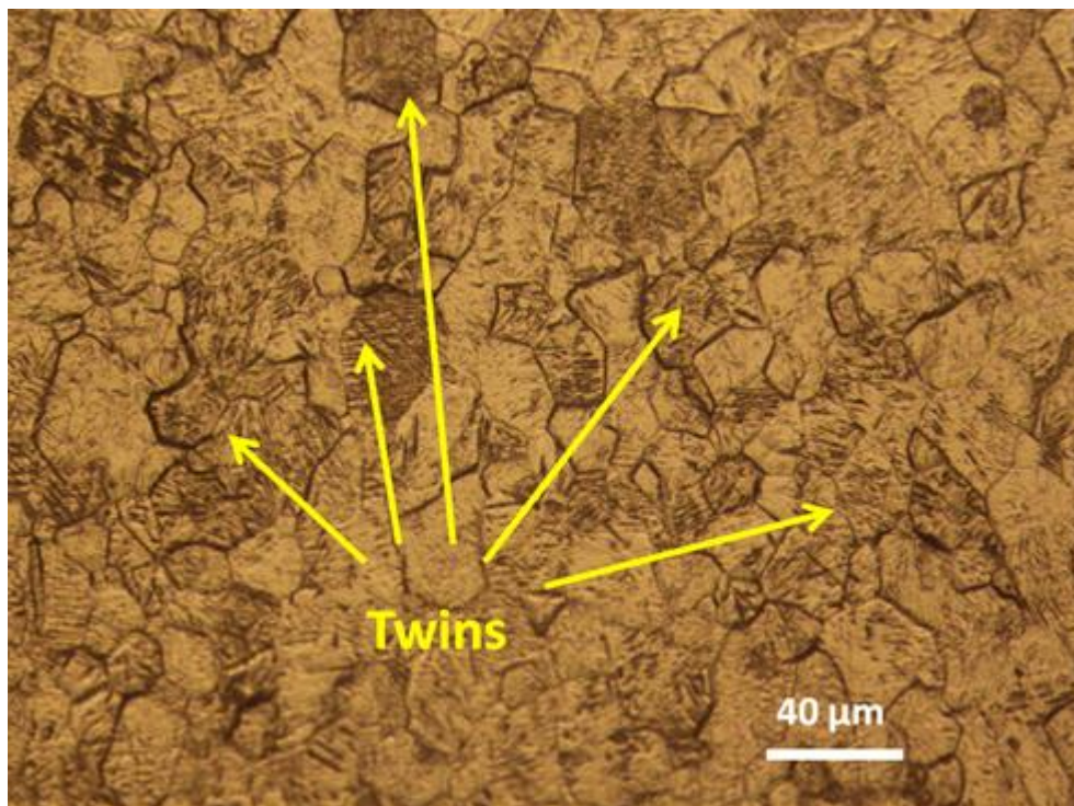
Fig. 4: The optical image of the microstructure of the as-received commercial pure titanium.
