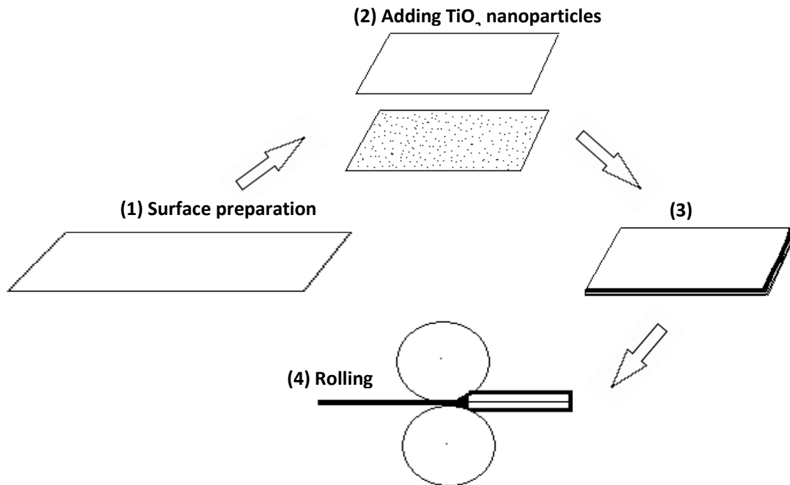
Fig. 1: The schematic illustration of the cold roll process for manufacturing the CP Ti/TiO 2 nanocomposite.
