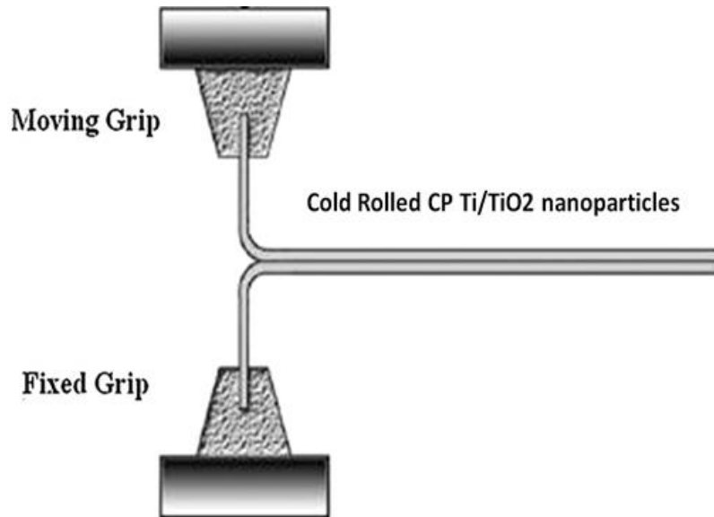
Fig. 2: The clamping configuration used in this study.
