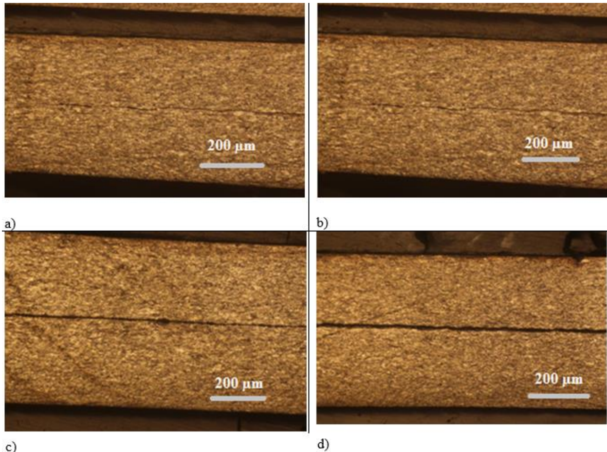
Fig. 7: Optical microscopy images of the RD-ND sheet of the cold rolled sheet: a) the monolithic CP-TiO 2 ; b) CP Ti/0.1wt.% nano-TiO 2 ; c) CP Ti/0.3wt.% nano-TiO 2 ; and d) CP Ti/0.5wt.% nano-TiO 2 .
