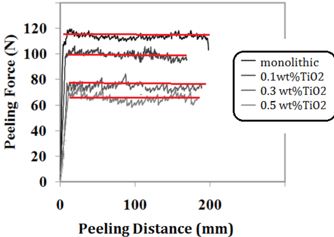
Fig. 5: The peeling test results.
