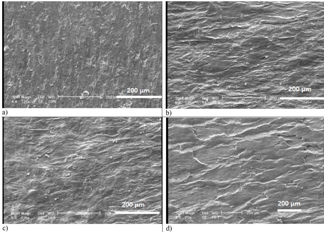
Fig. 6: SEM images of the peeled surfaces of samples including: a) the monolithic CP Ti; b) CP Ti/0.1wt.% nano-TiO 2 ; c) CP Ti/0.3wt.% nano-TiO 2 ; and d) CP Ti/0.5wt.% nano-TiO 2 .
