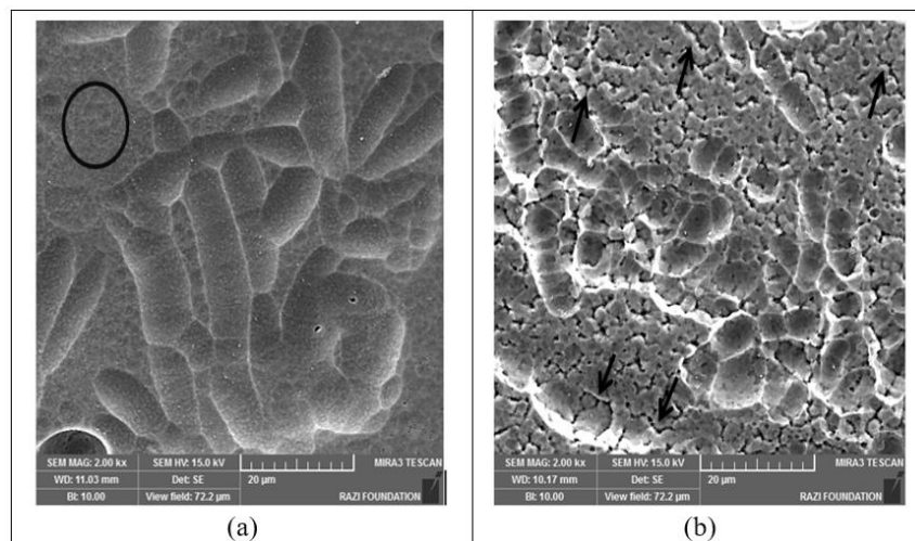
Fig. 2. SEM micrographs GeO 2 -PbO glasses after the quenching process; a) S.N.=1 and b) S.N.=3
